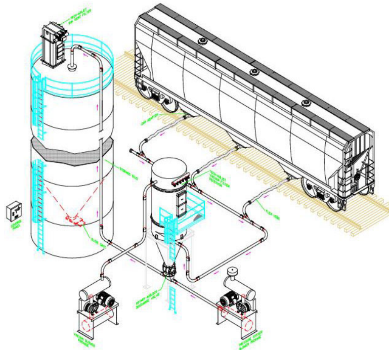
TYPICAL RAIL CAR UNLOADING SYSTEM
